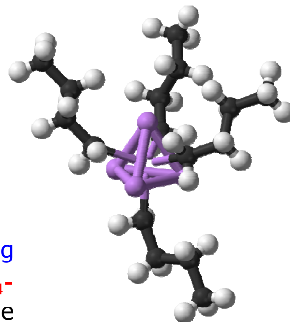
n -Butyllithium
